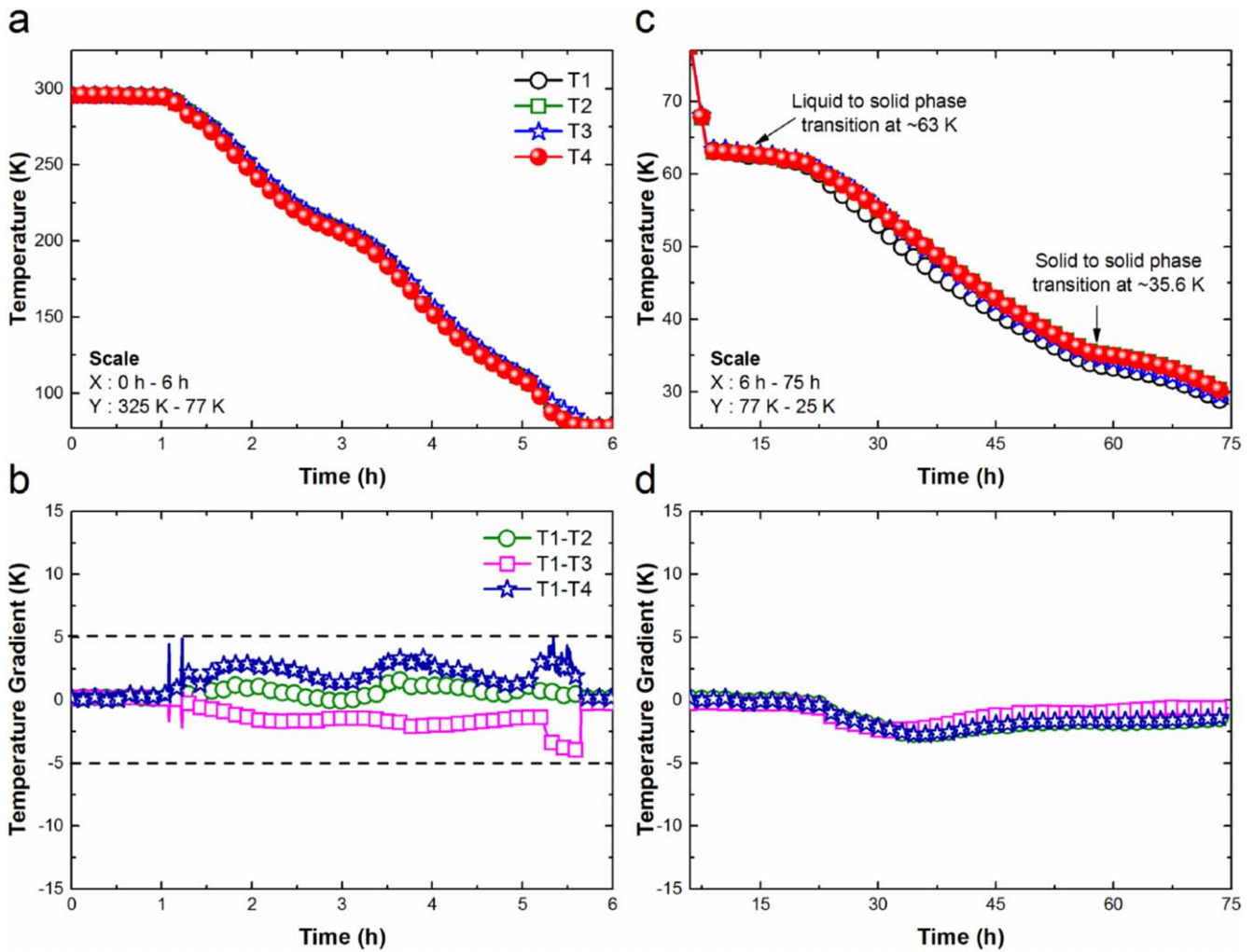
Figure 5. (a) Temperature versus time profiles from 300 to 77 K, (b) temperature gradient versus time profiles from 300 to 77 K, (c) temperature versus time profiles from 77 to 28.3 K, and (d) temperature gradient versus time profiles from 77 to 28.3 K during cool down of the coil in the SN 2 chamber. The cool down data are continuous in time. The legends in (a) and (c), and (b) and (d) are the same.
