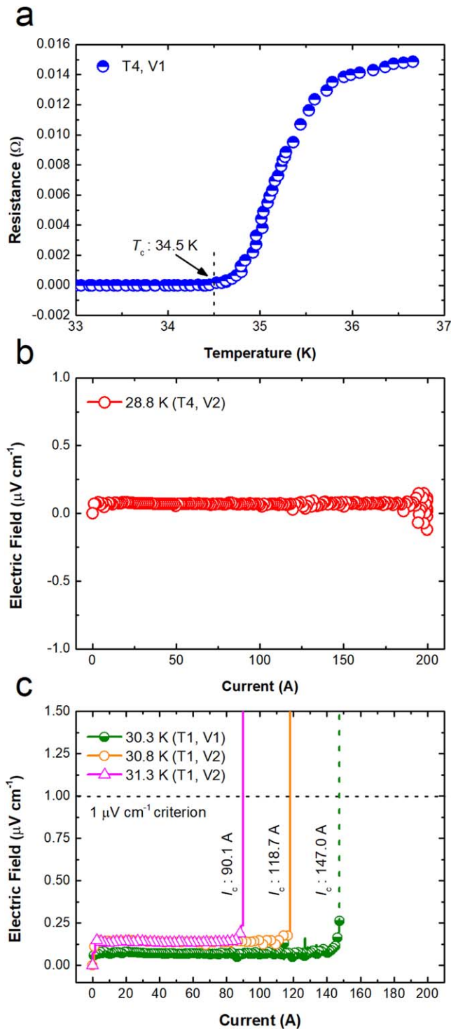
Figure 6. (a) Resistance versus temperature profile, electric field versus current characteristics (b) at 28.8 K (T4), and (c) at 30.3, 30.8 and 31.3 K (T1) for the racetrack coil. The dashed green line is an anticipated electric field line. The temperature sensor location T1 was at the top of the coil, and T4 was at the bottom of the coil. V1 and V2 represent the voltage taps across the entire coil and outer layer, respectively. The current ramp rate at 30.3 K was 0.5 \text{ A s}^{-1} , whereas, at 30.8 and 31.3 K, it was 1 \text{ A s}^{-1} .
