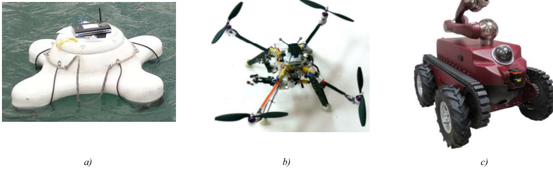
Figure 2. Photos of the vehicles comprising the heterogeneous robotic system: a) autonomous surface marine platform ( PladyPos made at UNIZG-FER), b) autonomous aerial vehicle ( ArduCopter Quad by jDrones) and c) autonomous ground vehicle ( Guardian by Robotnik) with a manipulator.
