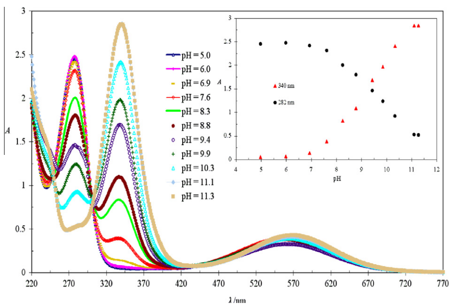
Fig. 2. pH-dependent UV–Vis spectra of the isolated \text{Na}(\text{PAM4})[\text{Fe}(\text{CN})_5(\text{PAM4})]\cdot\text{H}_2\text{O} in aqueous solutions at 25\text{ }^\circ\text{C} , c = 8 \times 10^{-5}\text{ M} , l = 0.1\text{ M} .
