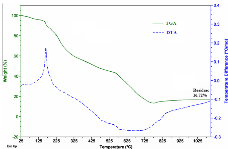
Fig. 3. TGA and DTA curves for \text{Na}(\text{PAM4})[\text{Fe}(\text{CN})_5(\text{PAM4})]\cdot\text{H}_2\text{O} .
