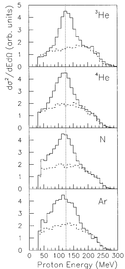
FIG. 2. The laboratory kinetic energy of protons with polar angles between 15^\circ and 25^\circ for ppp final states following the absorption of 239 MeV \pi^+ on {}^3\text{He} , {}^4\text{He} , N, and Ar. The dashed curves are the results of phase-space simulations, and the dotted line shows the average proton energy for free \pi^+p scattering.
