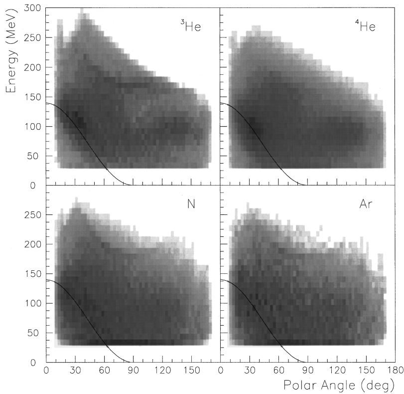
FIG. 1. Scatter plots of laboratory kinetic energy vs angle from the pion beam axis for ppp final states following the absorption of 239 MeV \pi^+ on {}^3\text{He} , {}^4\text{He} , N, and Ar. The solid line shows the kinematics for free \pi^+p scattering.
