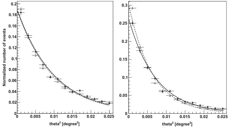
Fig. 12. \theta^2 distribution of the excess above 100 GeV (left panel) and above 300 GeV (right), for the Crab Nebula data sample (solid circles) and MC gamma simulations (open triangles). Fits with a 2D Gaussian distribution are shown with a solid (for data) or dashed (for MCs) line. A small 2D Gaussian mispointing with \sigma_{\text{mis}} = 0.014^\circ was added to the simulations.
