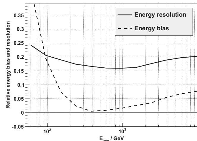
Fig. 11. Energy resolution (solid line) and the bias (dashed) obtained with the MC simulations of gamma-rays. Mild cuts are applied: Hadronness < 0.6 , \theta^2 < 0.03 .
