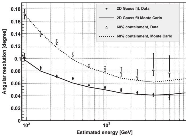
Fig. 13. Angular resolution as a function of the estimated energy obtained with the Crab Nebula data sample (points) and compared with the MC simulations (lines) for the 2D Gaussian fit (solid line, full circles) and the 68% containment radius (dashed line, empty triangles). A small 2D Gaussian mispointing with \sigma_{\text{mis}} = 0.014^\circ was added to the simulations.
