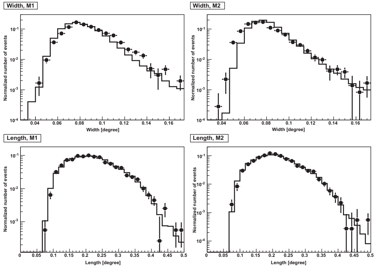
Fig. 10. Comparison of the width (top panels) and the length (bottom) parameters for MAGIC I (left panels) and MAGIC II (right). The solid line is computed with the MC gamma-rays, black points correspond to the gamma-rays excess, extracted with very loose cuts ( Hadronness < 0.9 , \theta^2 < 0.03 ) from the data sample. Only events with size > 200 phe are used.
