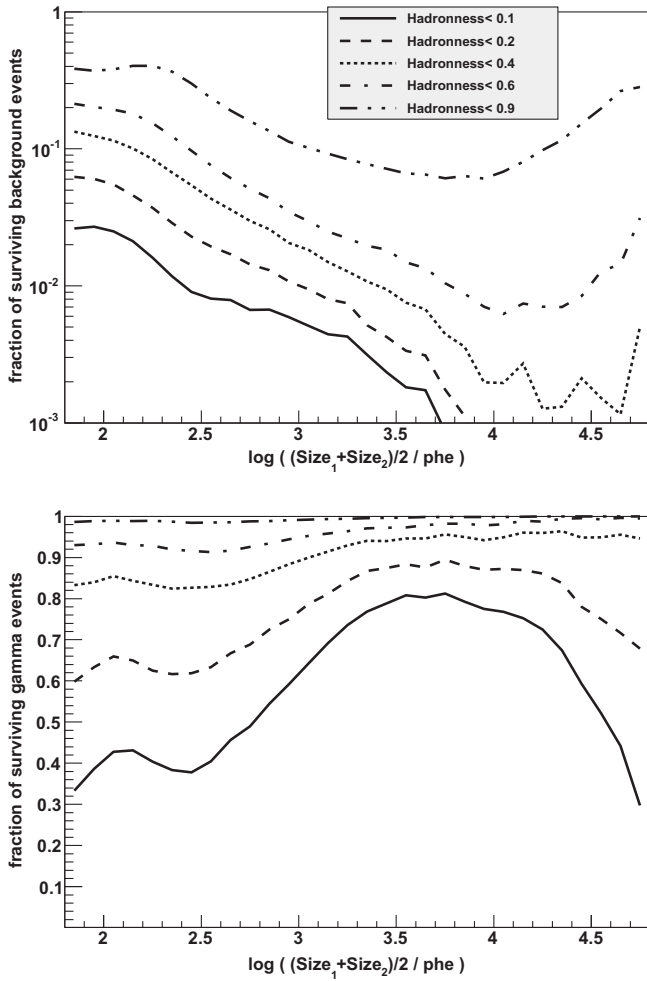
Fig. 3. Fraction of surviving background (data, top panel) and gamma-ray (MC, bottom panel) events. Different line styles are for different cuts: Hadronness < 0.1 (solid), < 0.2 (dashed), < 0.4 (dotted), < 0.6 (dot-dashed), and < 0.9 (dot-dot-dashed).
