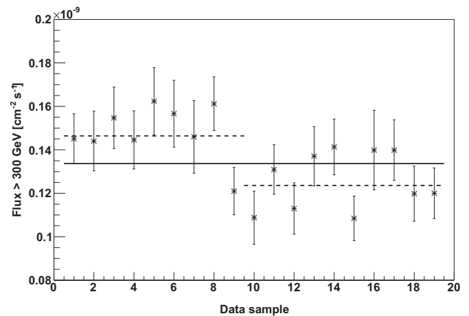
Fig. 19. Integrated flux above 300 GeV of the Crab Nebula, as the function of the data sample number. The solid horizontal line shows the mean flux in the whole period. The dashed lines show the mean fluxes in November 2009 (left) and January 2010 (right).
