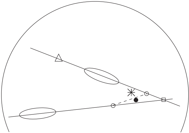
Fig. 5. Principle of the stereo DISP RF method. The crossing point of the main axes of the images is shown as an empty square, and the DISP RF reconstructed position from each telescope is an empty circle. The final reconstructed position (full circle) is a weighted average of those three points. The true source position is shown with a star. Open triangle shows the reconstructed source position for the top image if the head–tail discrimination failed.
