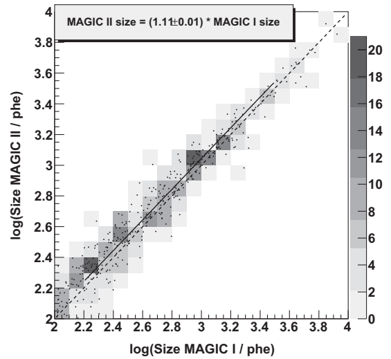
Fig. 8. Relation between size_2 and size_1 for gamma-ray events obtained with a Crab Nebula sample. Only events with a difference in the reconstructed impacts of both telescopes smaller than 10 m are considered. Individual events with Hadronness < 0.2 , \theta^2 < 0.01 and Impact parameters < 150 m are shown by black dots. The black, solid line shows the result of the fit, the dashed line corresponds to size_1 = size_2 .
