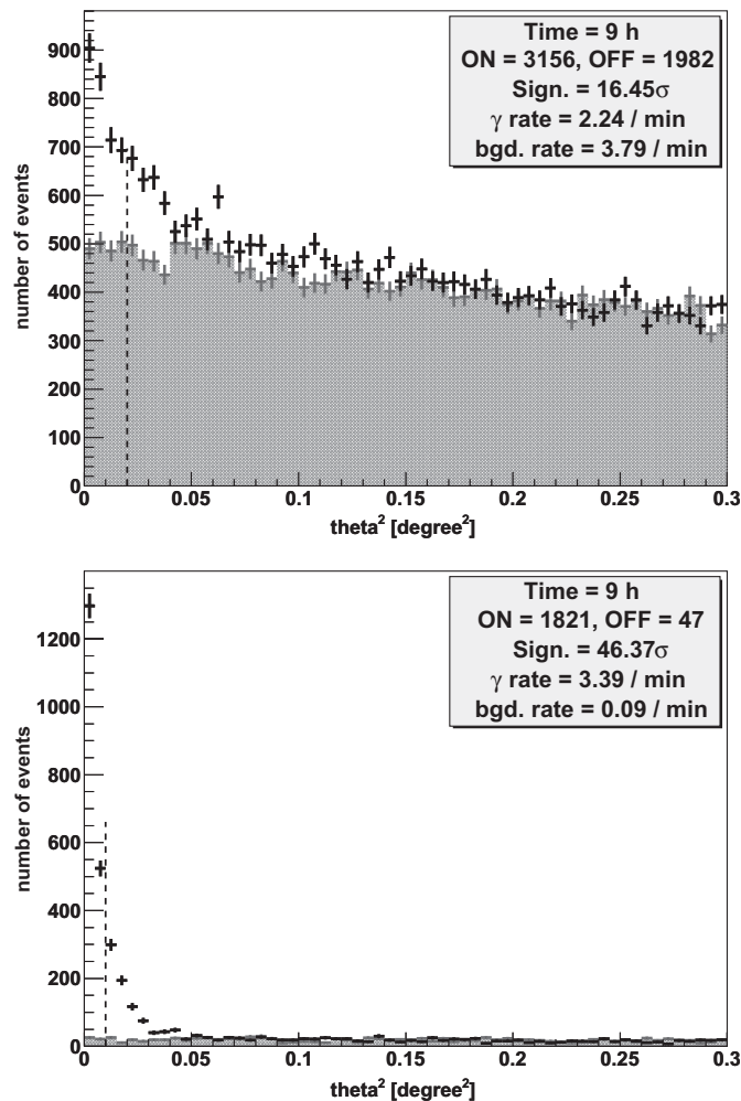
Fig. 6. \theta^2 distribution of the signal (black points) in the analyzed sample of the Crab Nebula data and the background estimation (grey shaded area). Estimated energy 60 \text{ GeV} < E_{\text{est}} < 100 \text{ GeV} (top panel) and E_{\text{est}} > 300 \text{ GeV} (bottom panel). The cut in \theta^2 used for the calculation of the number of ON and OFF events is shown with the dashed, vertical lines.
