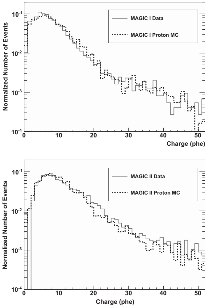
Fig. 7. Distribution of the smallest charge of the brightest 3NN cluster for data and Monte Carlo (continuous and dotted lines respectively) for MAGIC I (top panel) and MAGIC II (bottom).
