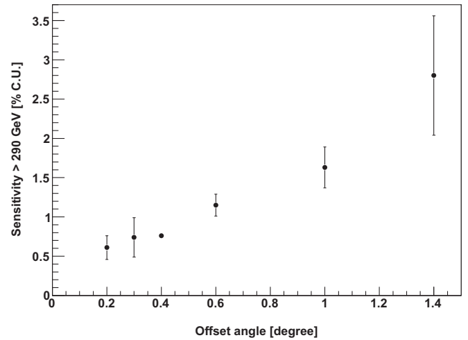
Fig. 18. Integral sensitivity above 290 GeV for the observation of a source at a different offset from the center of the camera. Each point is obtained with a small, dedicated sample of Crab Nebula data.
