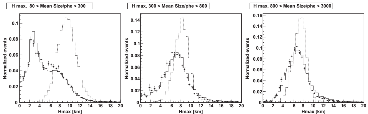
Fig. 2. Distribution of MaxHeight in different ranges of the mean size parameter for MC gamma-rays (dotted line), MC protons (full circles), and real data (solid line).
