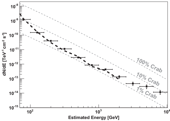
Fig. 16. Differential sensitivity of the MAGIC Stereo system. We compute the flux of the source in a given energy range for which N_{\text{excess}}/\sqrt{N_{\text{bkg}}} = 5 , N_{\text{excess}} > 10 , N_{\text{excess}} > 0.05N_{\text{bkg}} after 50 h of effective time for the data (black points), and the MC (dashed line). The horizontal error bars represent the size of the bins in estimated energy (5 bins per decade). For comparison, fractions of the Crab Nebula spectrum are plotted with the thin dashed gray lines.
