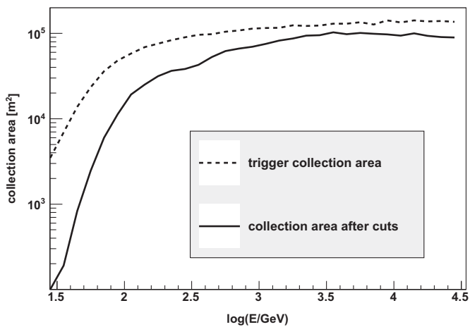
Fig. 4. Gamma-ray collection area of the MAGIC telescopes (MC simulations) at the trigger level (dashed line) and after all analysis cuts (image cleaning of both images, size > 50 in both telescopes, gamma/hadron and \theta^2 cuts).
