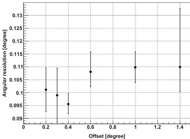
Fig. 17. Angular resolution (defined as the 68% containment radius) for gamma-rays with energy above 200 GeV for the observation of a source at a different offset from the center of the camera. Each point is obtained with a small, dedicated sample of Crab Nebula data.
