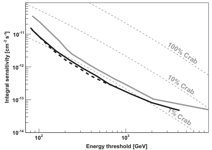
Fig. 15. Integral sensitivity of the MAGIC Stereo system, i.e. the flux of a source above a given energy for which N_{\text{excess}}/\sqrt{N_{\text{bgd}}} = 5 after 50 h of effective observation time for MAGIC Stereo (black, solid – data, dashed – MCs) compared with the MAGIC I telescope (solid gray line). For comparison, fractions of the integral Crab Nebula spectrum are plotted with the thin, dashed, gray lines.
