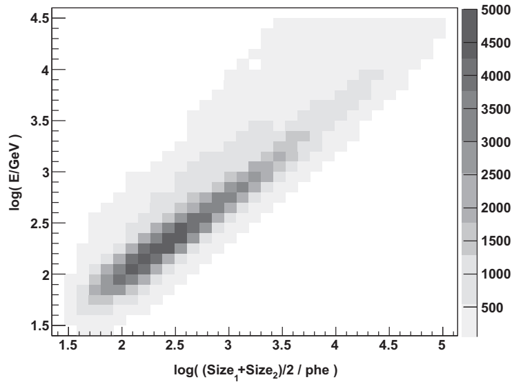
Fig. 1. Correlation between the mean size of a gamma-ray event and its energy obtained with MC simulations.
