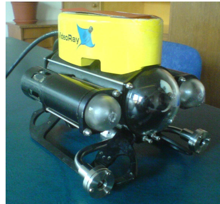
Fig. 1. VideoRay ROV with vision-based distance keeping sensor
