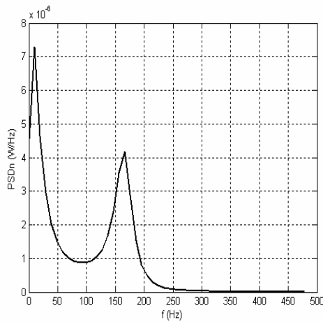
Fig.2. Power Spectral Density of noise
