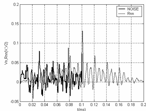
Fig. 1. The noise and its autocorrelation
