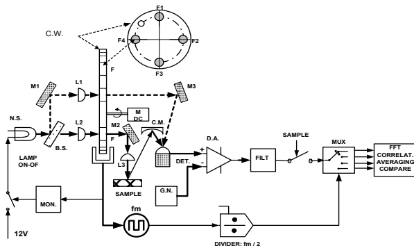
Fig. 3. Equipment for measuring moisture on sample
