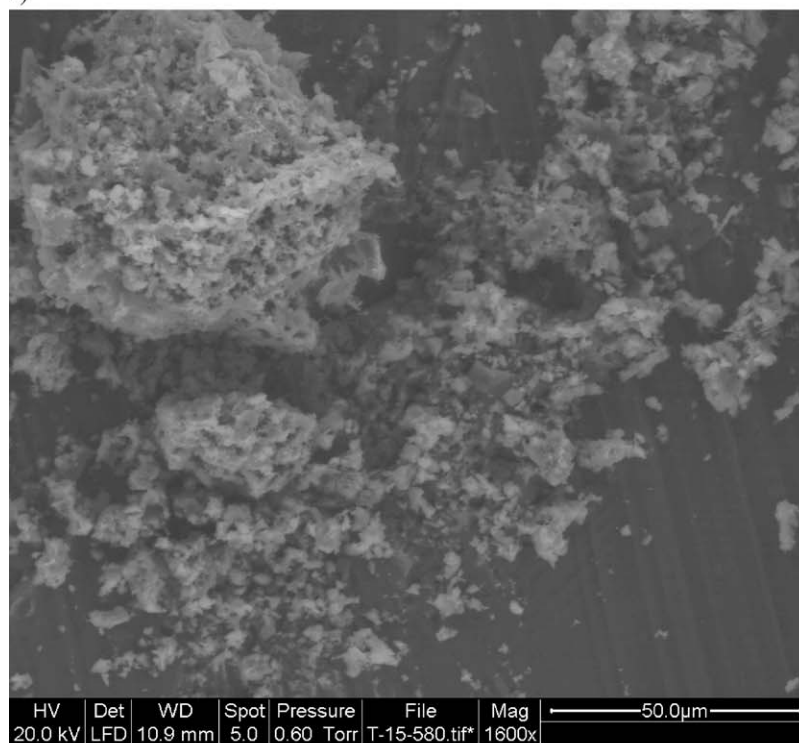
Figure 9. Scanning electron micrographs obtained by analyzing a powder of sample T-0-580 (a) and sample T-15-580 (b).
