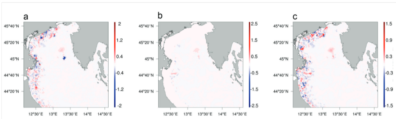
Fig. 2: The differences in sea temperatures after 15 days (30/11/2015) of continuous discharge (started on 14/11/2015) from the potential offshore LNG terminal Istria in the northern Adriatic Sea at: a. the sea surface, b. 25 m depth, and c. the seabed, compared to the normal situation (without discharges) in November (the autumn period).
