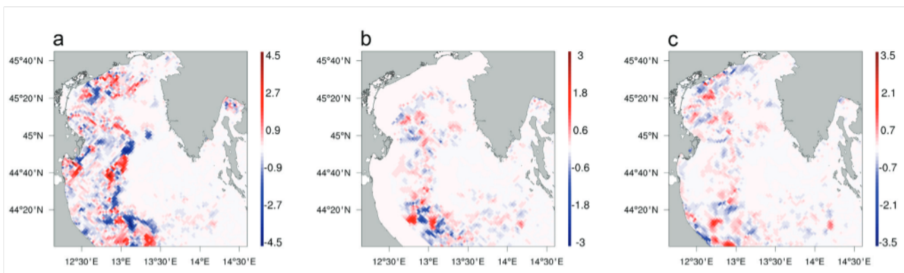
Fig. 3: The differences in sea temperatures after 32 days (16/12/2015) of continuous discharge (started on 14/11/2015) from potential offshore LNG terminal Istria in the northern Adriatic Sea at: a. the sea surface, b. 25m depth, and c. the seabed, compared to the normal situation (without discharges) in December (the autumn period).
