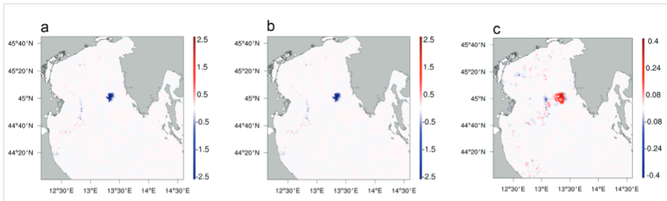
Fig. 1: The differences in sea temperatures after 5 days (on 20/11/2015) of continuous discharge (started on 14/11/2015) from the potential offshore LNG terminal Istria in the northern Adriatic Sea at: a. the sea surface, b. 25 m depth, and c. the seabed, compared to the normal situation (without discharges) in November (the autumn period).
