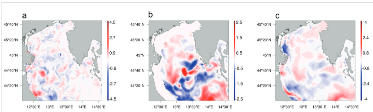
Fig. 6: The differences in sea temperatures after 3 months (06/08/2016) of continuous discharge (started on 02/05/2016) from potential offshore LNG terminal Istria in the northern Adriatic Sea at: a. the sea surface, b. 25m depth, and c. the seabed, compared to the normal situation (without discharges) in August (the spring-summer period).
