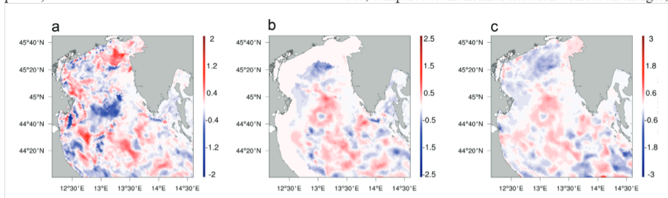
Fig. 4: The differences in sea temperatures after 17 days (20/05/2016) of continuous discharge (started on 02/05/2016) from the potential offshore LNG terminal Istria in the northern Adriatic Sea at: a. the sea surface, b. 25m depth, and c. the seabed, compared to the normal situation (without discharges) in May (the spring-summer period).
