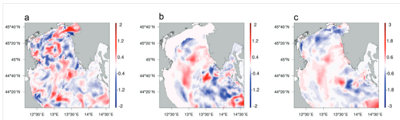
Fig. 5: The differences in sea temperatures after 45 days (17/06/2016) of continuous discharge (started on 02/05/2016) from potential offshore LNG terminal Istria in the northern Adriatic Sea at: a. the sea surface, b. 25m depth, and c. the seabed, compared to the normal situation (without discharges) in June (the spring-summer period).
