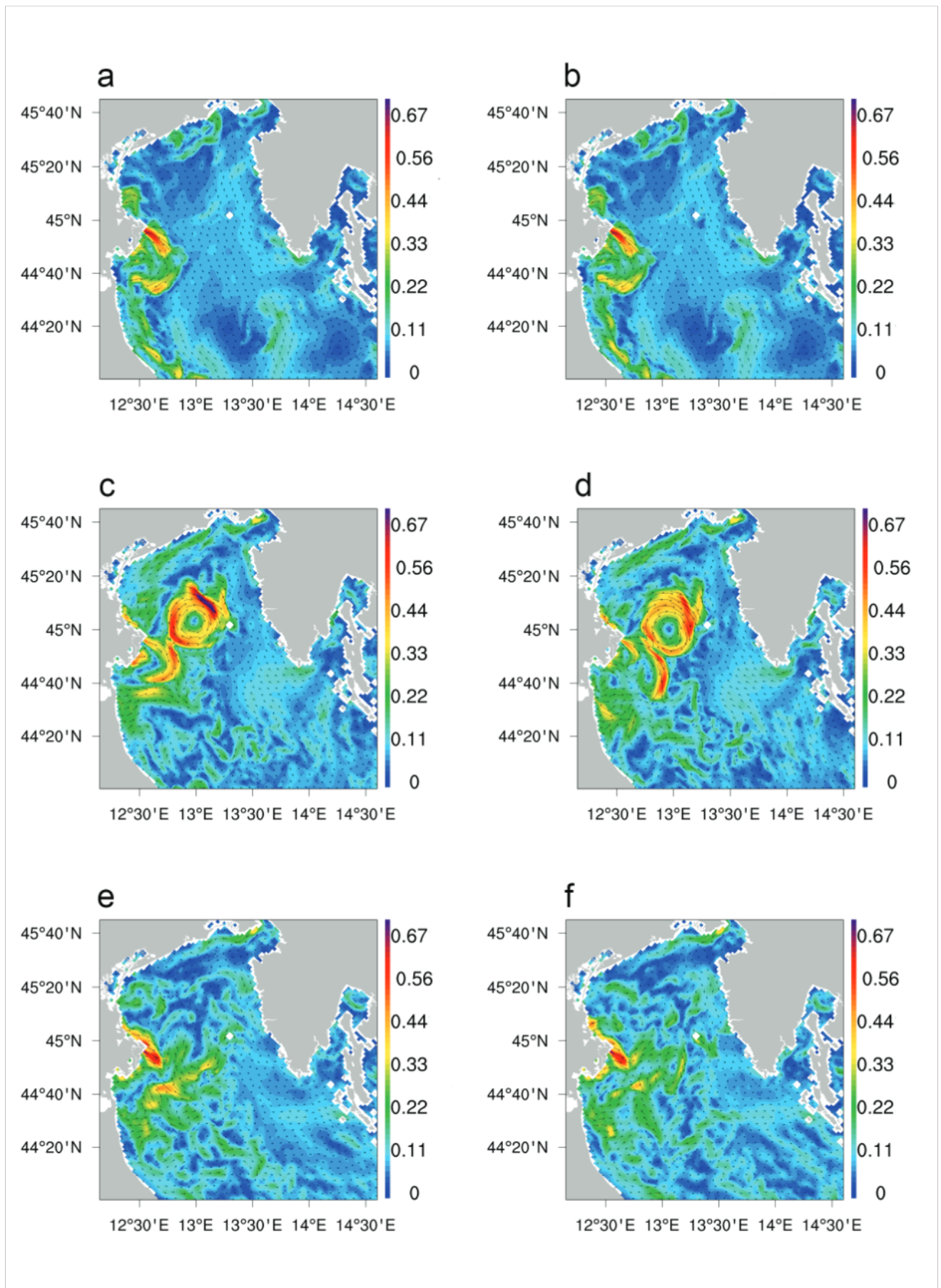
Fig. 7: Sea currents at the sea surface: a. without discharge on 03/12/2015, b. after 18 days of continuous discharge on 03/12/2015, c. without discharge on 01/01/2016, d. after 1.5 months of continuous discharge on 01/01/2016, e. without discharge on 19/02/2016, and f. after 3 months of continuous discharge on 19/02/2016 in the northern Adriatic Sea.
