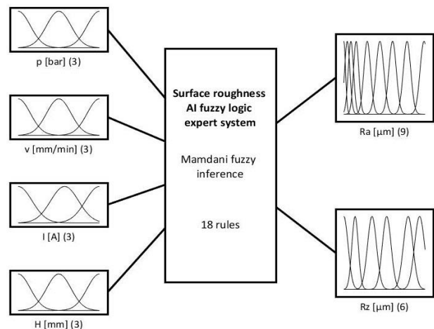
Figure 4. AI fuzzy logic system for modeling and prediction surface roughness response
