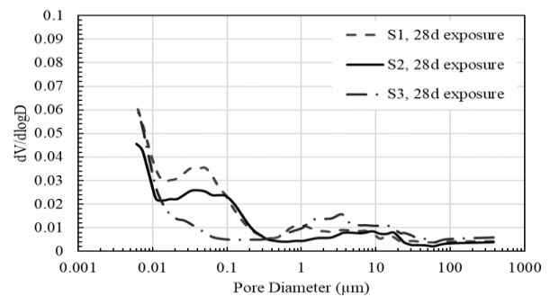
Fig. 9. Log differential curves of S1, 2 and S3 mixes after 28 days of exposure to accelerated carbonation.
