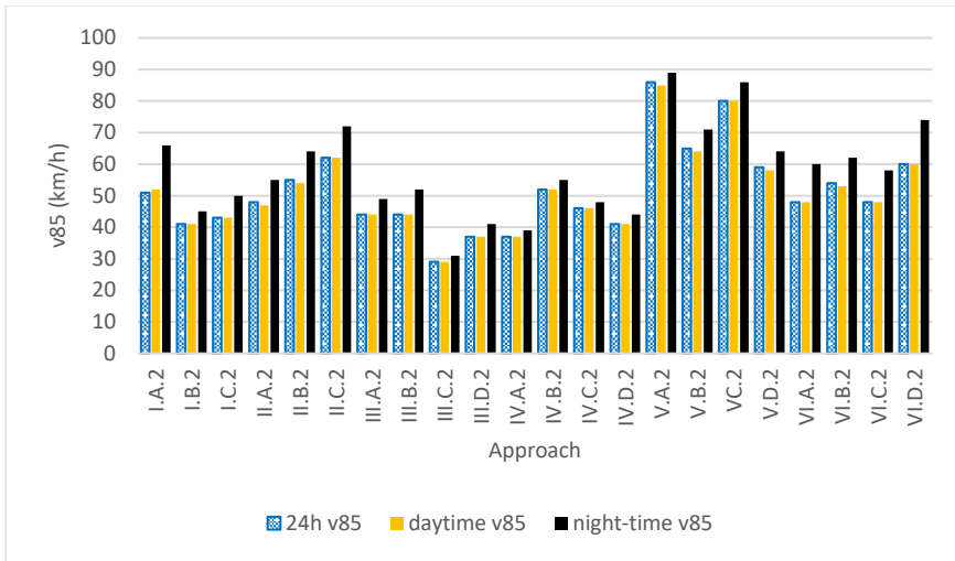
Figure 2. Comparison of v 85 approaching speed at Position 2.
