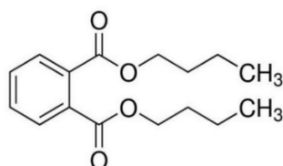
Figure 1. Structure of dibutyl phthalate
