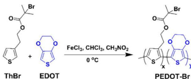
Figure 1. Reaction scheme of macroinitiator synthesis
