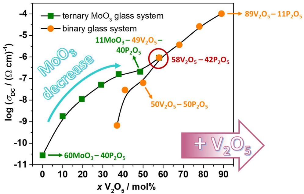
Figure 1. Polaronic conductivity as a function of V 2 O 5 content for the binary and ternary glass series.
