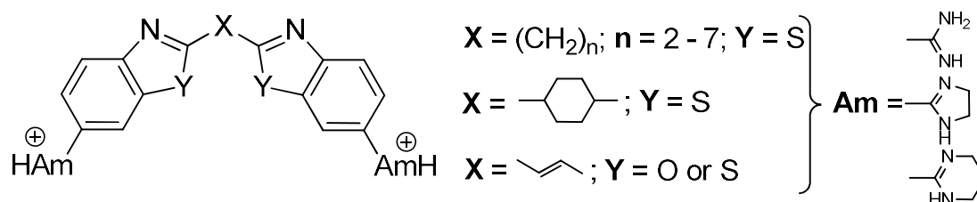
Figure 1: The structures of dicationic bis-6-amidinobenzothiazole and benzoxazole derivatives
