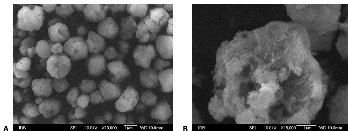
Figure 1. SEM images of FAU type zeolite treated with CTAB (A) and the one etched with \text{NaOH}_{(\text{aq})}
