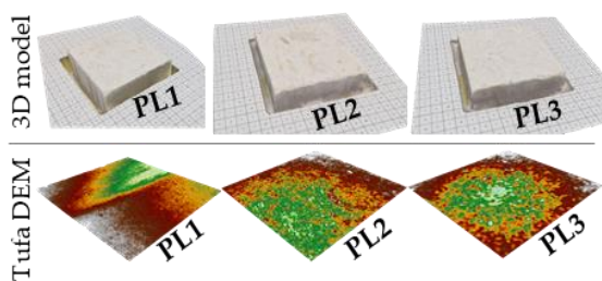
Figure 13: Derived reference 3D models and tufa DEMs on micro level of research.
