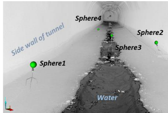
Figure 12: Recognized spheres at eighth scan station.
