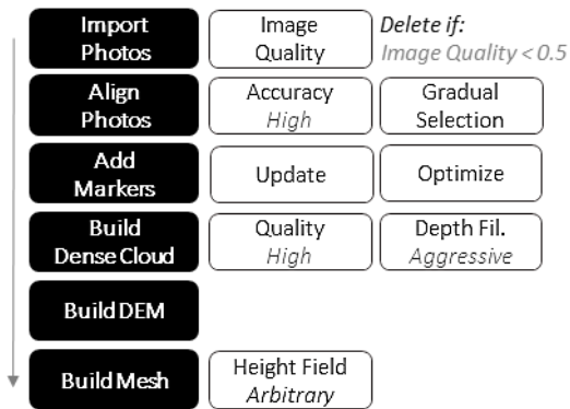
Figure 9: Image processing in Agisoft Metashape.
