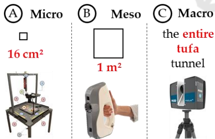
Figure 4: Sensors used in three level of research at tufa tunnel.
