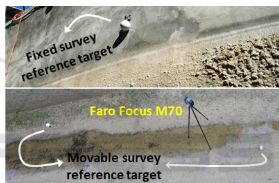
Figure 8: Terrestrial laser scanning of tufa tunnel.
