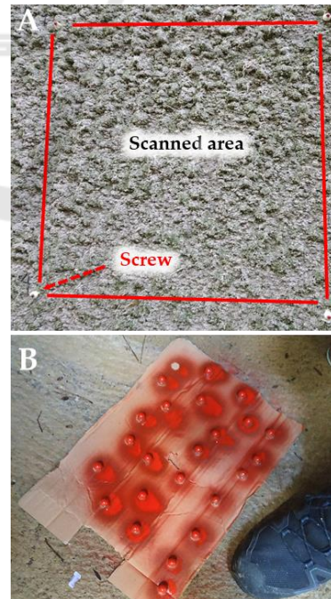
Figure 6: (A) Square surfaces scanned using Artec Eva; (B) colored caps used as GCPs.
