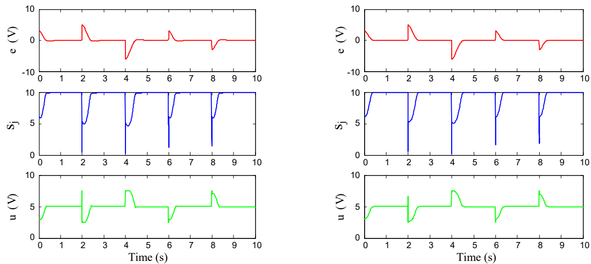
Figure 7. Simulation results for position control. Position error e and change of position error \Delta e are the input variables.
