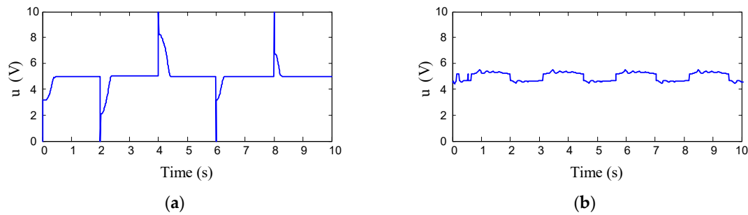
Figure 8. Experimental results for position control with two input variables e and \Delta e : (a) step inputs, (b) sinusoidal inputs.
