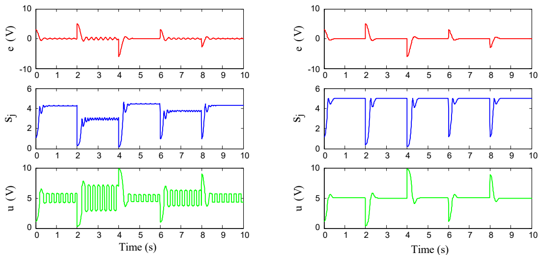
Figure 6. Simulation results for position control. Position error e is the input variable.
