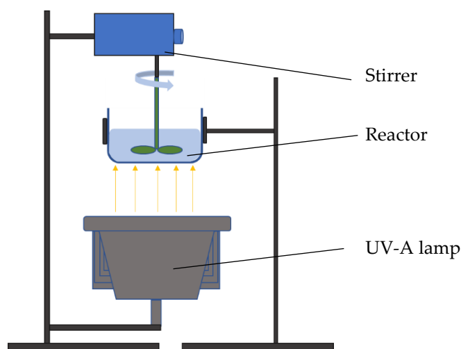
Figure 11. The reactor for photocatalytic measurements.
