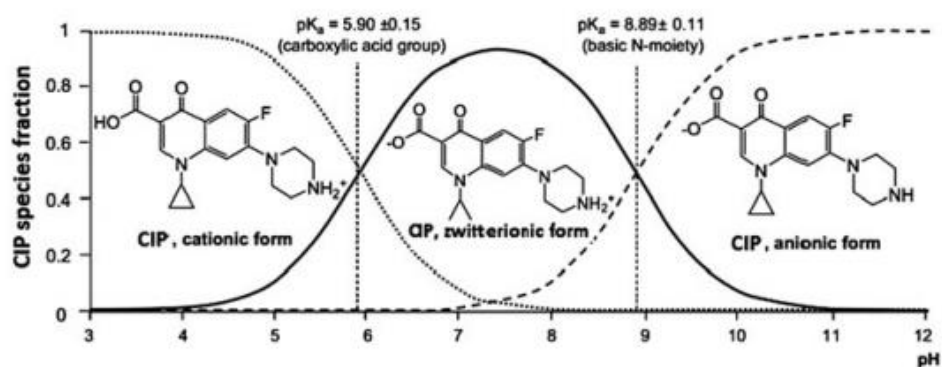
Figure 12. Molecular structure of CIP and its ionic forms as a function of pH and pK_a values [56].
