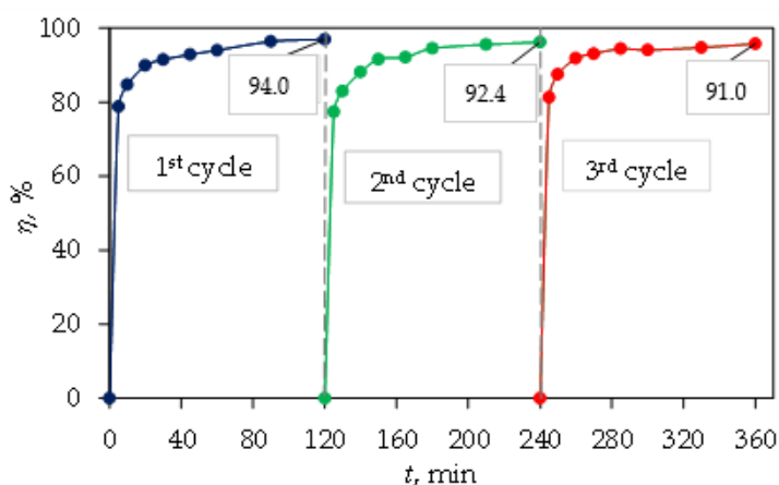
Figure 10. Reusability efficiencies of the ternary core-shell \text{Fe}_3\text{O}_4/\text{SiO}_2/\text{TiO}_2 photocatalyst for three consecutive cycles.
