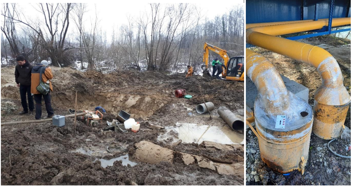
Figure 4. a) Re-construction works on water pipeline at Cepeliš that is crossed by regional Pokupsko Fault (CREDIT: HGI EQ Team); b) Temporarily repaired Gas pipeline damaged because of sinistral coseismic displacement of Galdovo Bridge.
