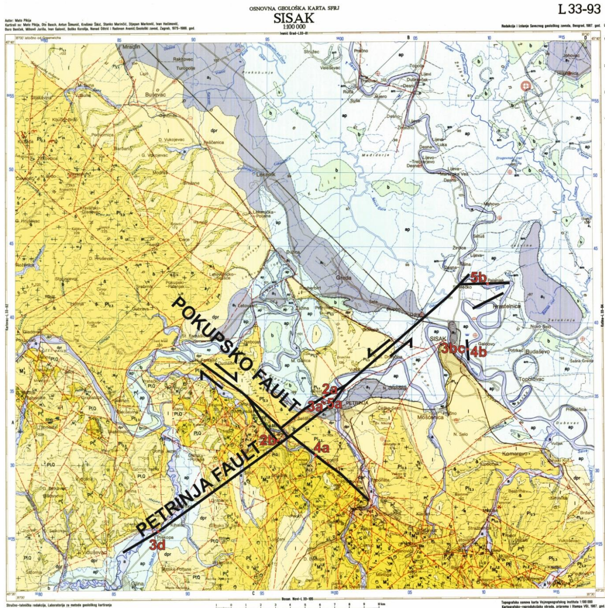
Figure 1. a) Geological map [3] showing the main activated faults (thick black lines) during the Petrinja 2020 sequence [1]. Red dots and numbers mark locations of the other figures.
