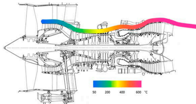
Figure 22. Typical casing temperature profile along an aeroengine with high bypass ratio [155].
