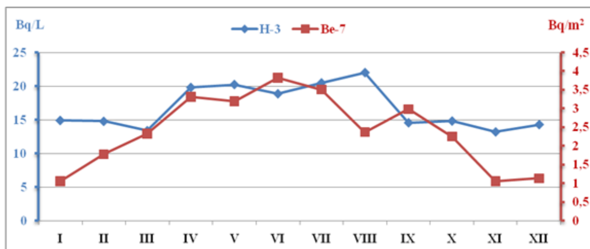
Figure 3. Monthly indices of ^3\text{H} and ^7\text{Be} activity concentration during 1995-2005.
