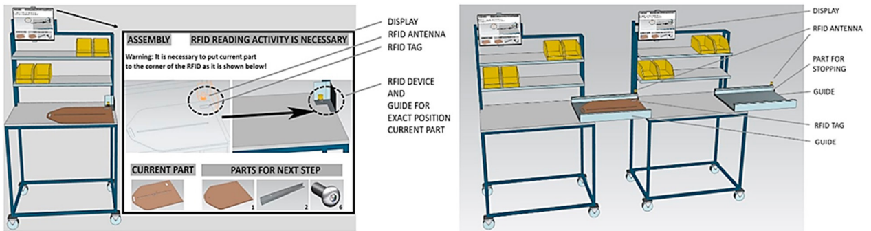
Fig. 3. Working station equipped with RFID reader and guidance displayed on tablet (left side) and design of guide for one working station equipped with RFID reader (right side)
