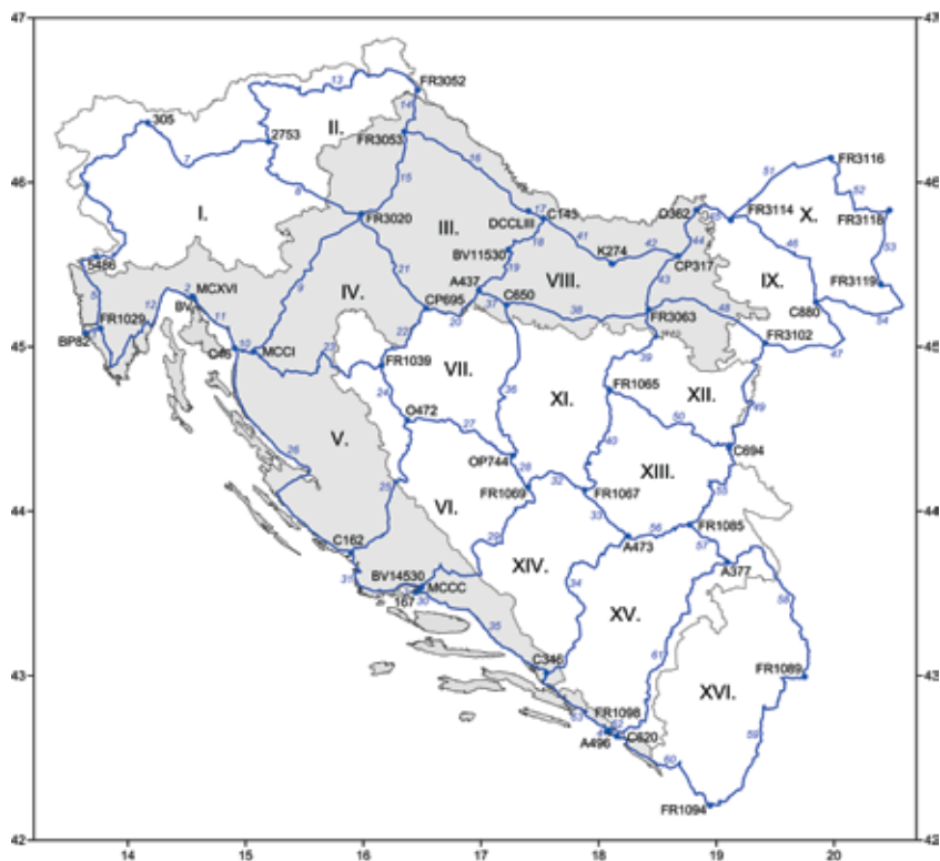
Figure 6. IINVT levelling network at territory of the Republic of Croatia.
