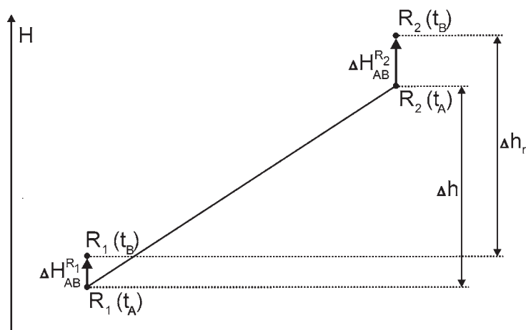
Figure 5. Height difference reduction regarding epoch's t_A i t_B .
