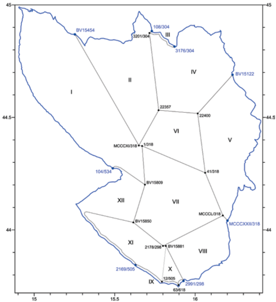
Figure 8. Scheme of II order levelling network geometrical configuration – loop no. V.
