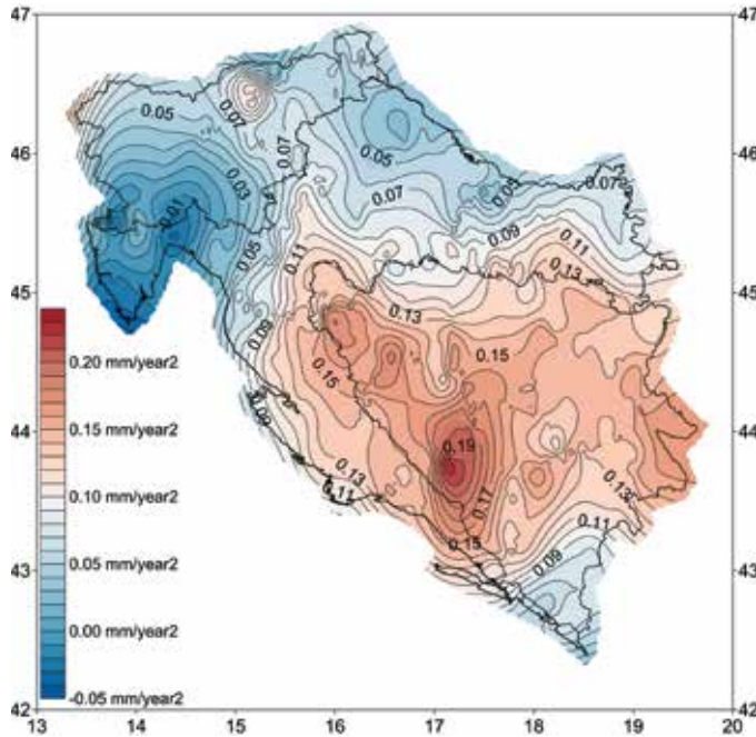
Figure 4. Grid model - parameter \alpha .
