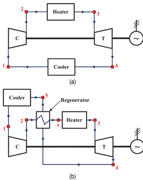
Figure 1 Scheme of the CO 2 closed-cycle gas turbine with marked operating points required for the analysis: (a) Base process; (b) Process with the regenerator
