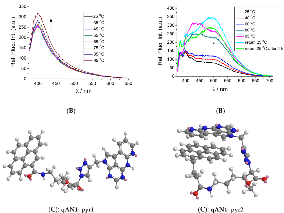
Figure 3. Comparison of qAN1-pyr1 and qAN1-pyr2 fluorescence spectra ( \lambda_{exc} = 350 nm, c = 8 \mu M, pH 7.0, I = 0.05 M): (A) Concentration dependence of emission; (B) temperature dependence of emission. (C) Schematic presentation of intramolecular organization of qAN1-pyr1 and qAN1-pyr2 according to UV/Vis and fluorimetric data (supported by preliminary energy-minimization done in vacuum, Suppl. Info, Figure S19).
