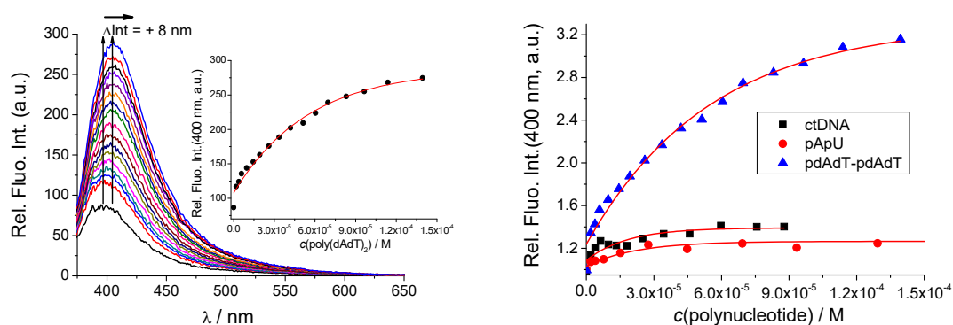
Figure 4. (Left): Fluorimetric titration of qAN1-pyr1 ( c = 1 \times 10^{-6} M; \lambda_{\text{exc}} = 350 nm) with poly (dAdT) 2 ; (Right): titrations with ds-DNA/RNA at 400 nm. Performed in sodium cacodylate buffer (pH 7, I = 0.05 M) at room temperature.
