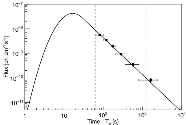
FIG. 1: Intrinsic LC model. The points represent the \gamma -ray flux measured by MAGIC above 0.3 TeV, while the full line represents the LC model reported in [19]. The vertical dashed lines represent the bounds of the time interval considered in our analysis.
