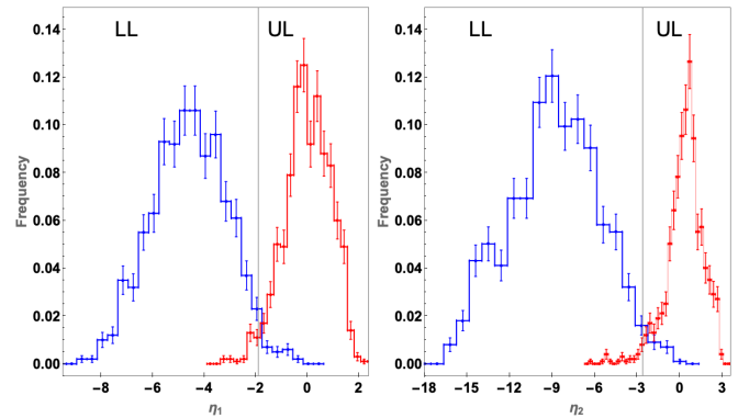
FIG. 5: Distribution of lower (blue) and upper limits (red) for the linear (left) and quadratic case (right), obtained from reshuffled-bootstrapped samples and using the theoretical assumption for the intrinsic LC. The vertical lines indicate respective bias values.
