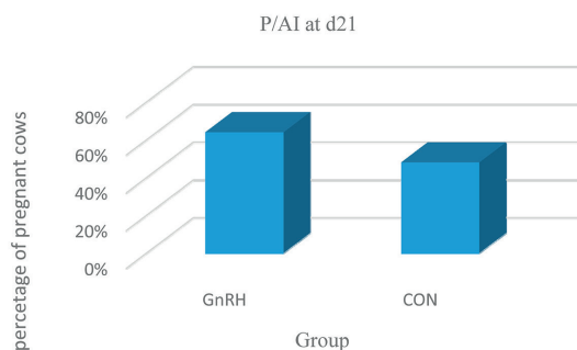
Figure 1. Percentage of pregnant cows at d 21. Cows were synchronized with PGF_2\alpha and AI-ed at detected estrus. At d 5 after AI, cows were treated with 0.008 mg Buserelin – a GnRH agonist (GnRH group) while the remaining cows (CON group) were left untreated. Pregnancy diagnoses was done at d 21 and confirmed d 30 after AI
