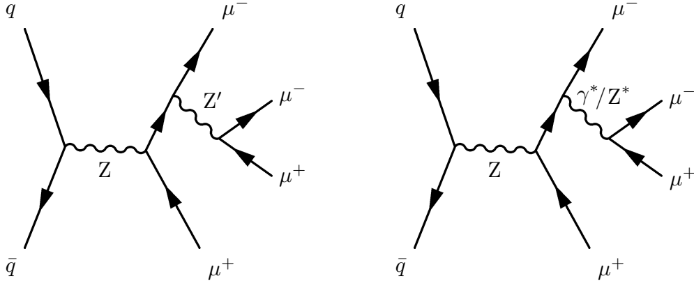
Figure 1: Leading order Feynman diagrams for the signal process (left) and the dominant background process (right), where in each diagram the four-muon final state originates from annihilation.
