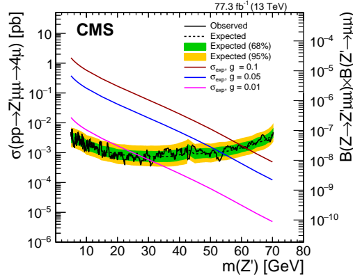
Figure 5: Expected and observed 95% CL limits on the product of the Z'\mu\mu production cross section and branching fraction (left y-axis) and \mathcal{B}(Z \rightarrow Z'\mu\mu)\mathcal{B}(Z' \rightarrow \mu\mu) (right y-axis). The dashed black curve is the expected upper limit, with one and two standard-deviation bands shown in green and yellow, respectively. The solid black curve is the observed upper limit. The colored lines show the predicted cross section times branching fraction (left y-axis) and \mathcal{B}(Z \rightarrow Z'\mu\mu)\mathcal{B}(Z' \rightarrow \mu\mu) (right y-axis) as a function of m(Z') for three different coupling strengths, chosen for illustration. The \mathcal{B}(Z' \rightarrow \mu\mu) is taken to be 1/3 to derive the theoretical predictions.
