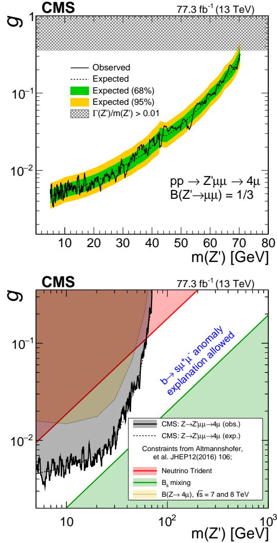
Figure 6: Top: Expected and observed 95% CL limits on the gauge coupling strength g as a function of m(Z') . The dashed black curve is the expected upper limit, with one and two standard-deviation bands shown in green and yellow, respectively. The solid black curve is the observed upper limit. The \mathcal{B}(Z' \rightarrow \mu\mu) = 1/3 is used to derive the upper limits. The hatched area shows the region where the narrow width approximation is no longer valid. Bottom: comparison with other experiments sensitive to the same parameter space, with shaded regions being excluded as described in the text. These three constraints are adapted from Ref. [13].
