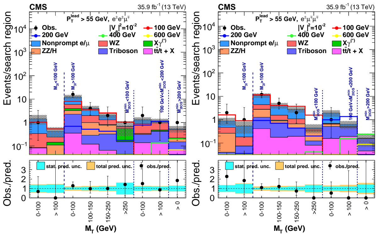
Figure A.3: Expanded version of Fig. 1, showing the observed and expected event yields in the high-mass region without an OSSF pair, for events with at least 2 electrons (left) and 2 muons (right). Contributions from various possible signals are shown for comparison.
