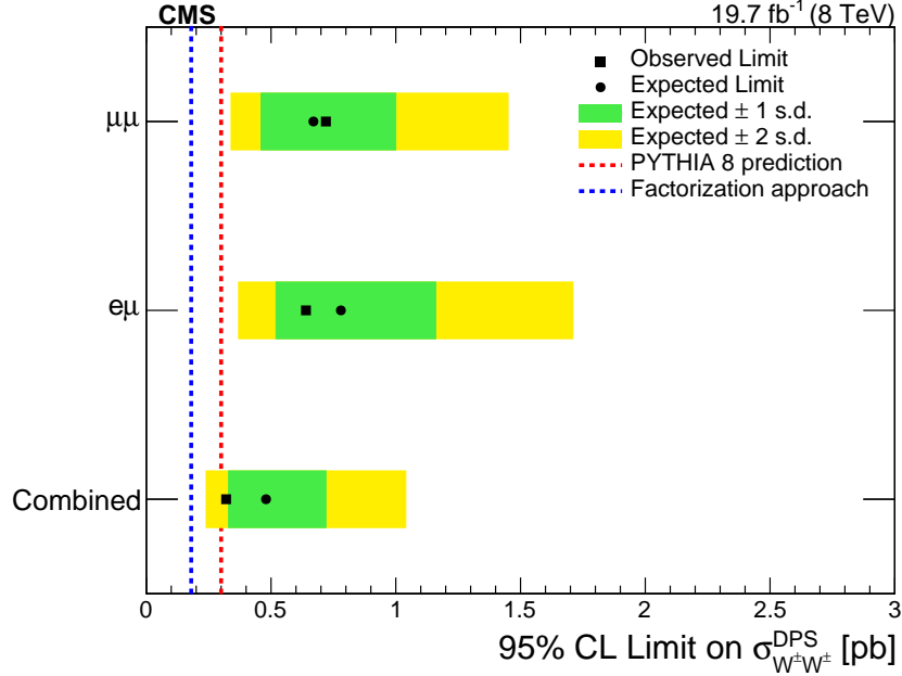
Figure 5: Expected and observed 95% CL upper limits on the same-sign \sigma_{W^{\pm}W^{\pm}}^{\text{DPS}} for the dimuon and electron-muon final states, along with their combination. The predicted values of \sigma_{W^{\pm}W^{\pm}}^{\text{DPS}} from PYTHIA8 and from the factorization approach [21] are also shown.
