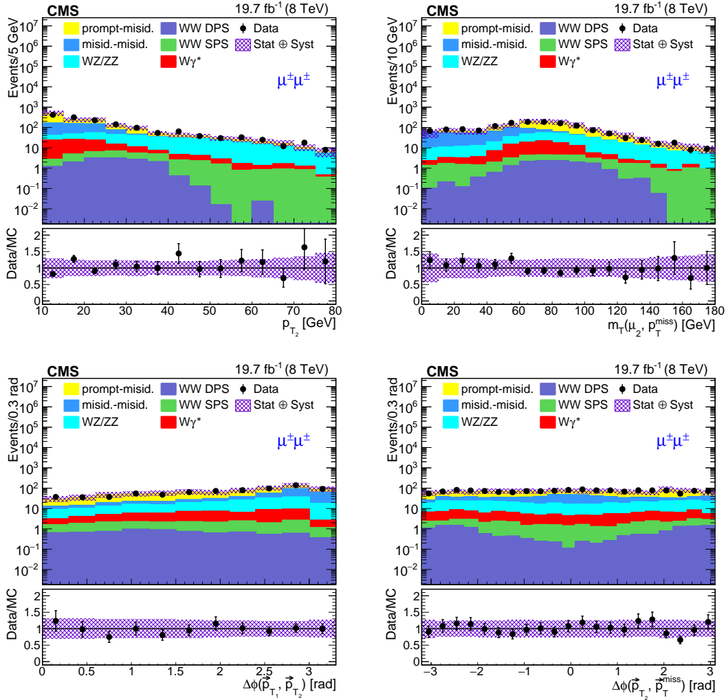
Figure 2: Distributions of the p_{T2} (top-left), m_T(\mu_2, p_T^{\text{miss}}) (top-right), \Delta\phi(\vec{p}_{T1}, \vec{p}_{T2}) (bottom-left), and \Delta\phi(\vec{p}_{T2}, \vec{p}_T^{\text{miss}}) (bottom-right) variables for the dimuon channel, after the same-sign WW selection criteria have been applied. The data are represented by the black dots and the shaded histograms represent the predicted signal and background processes normalized according to the estimated cross sections and the luminosity. For each individual distribution, the bottom panels show the ratio of the number of events observed in the data to that predicted by the simulation, along with the associated statistical uncertainty. The hatched bands in all cases represent the sum of the systematic and statistical uncertainties of the simulated samples, added in quadrature.
