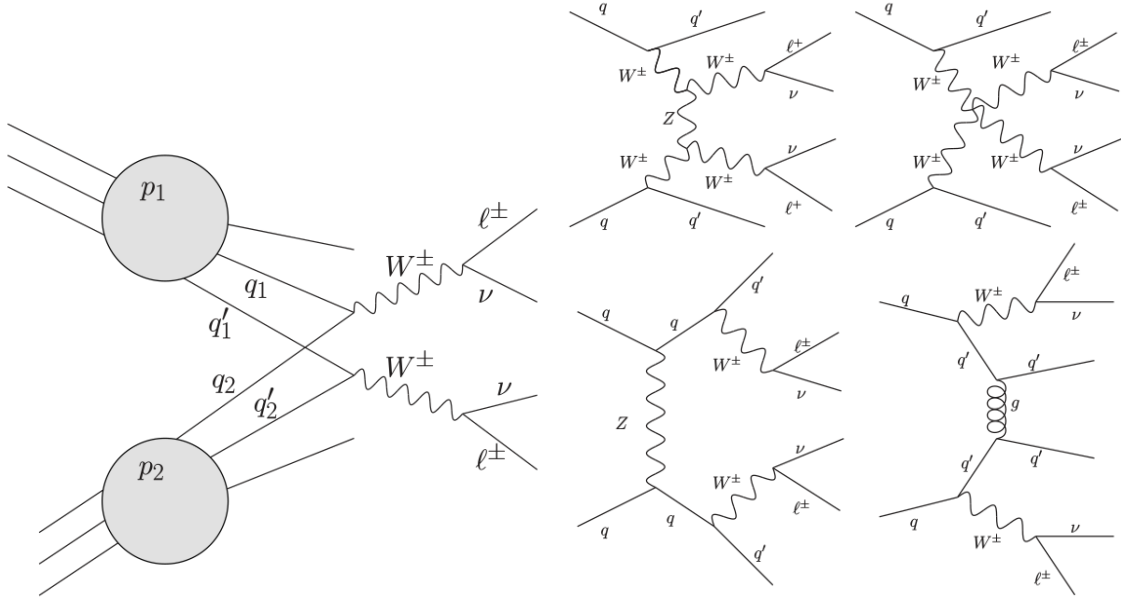
Figure 1: Schematic diagrams corresponding to the production of a same-sign W boson pair via the DPS process (left) and via SPS processes (right).
