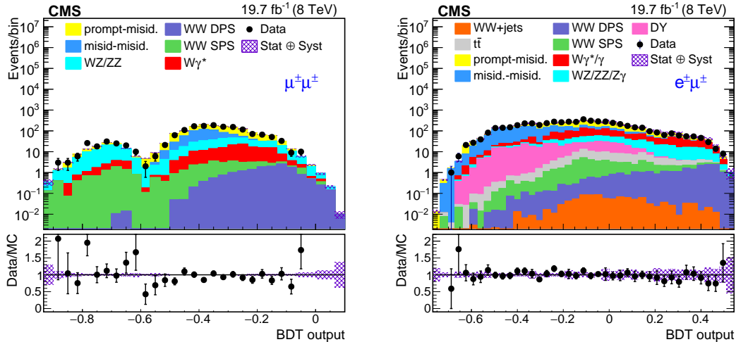
Figure 4: Distribution of the BDT discriminant, for the dimuon channel (left) and for the electron-muon channel (right). The data are represented by the black dots and the shaded histograms represent the pre-fit signal and post-fit background processes. The bottom panels show the ratio of data to the sum of all signal and background contributions. The hatched bands represent the post-fit uncertainty, which includes both the statistical and systematic components.
