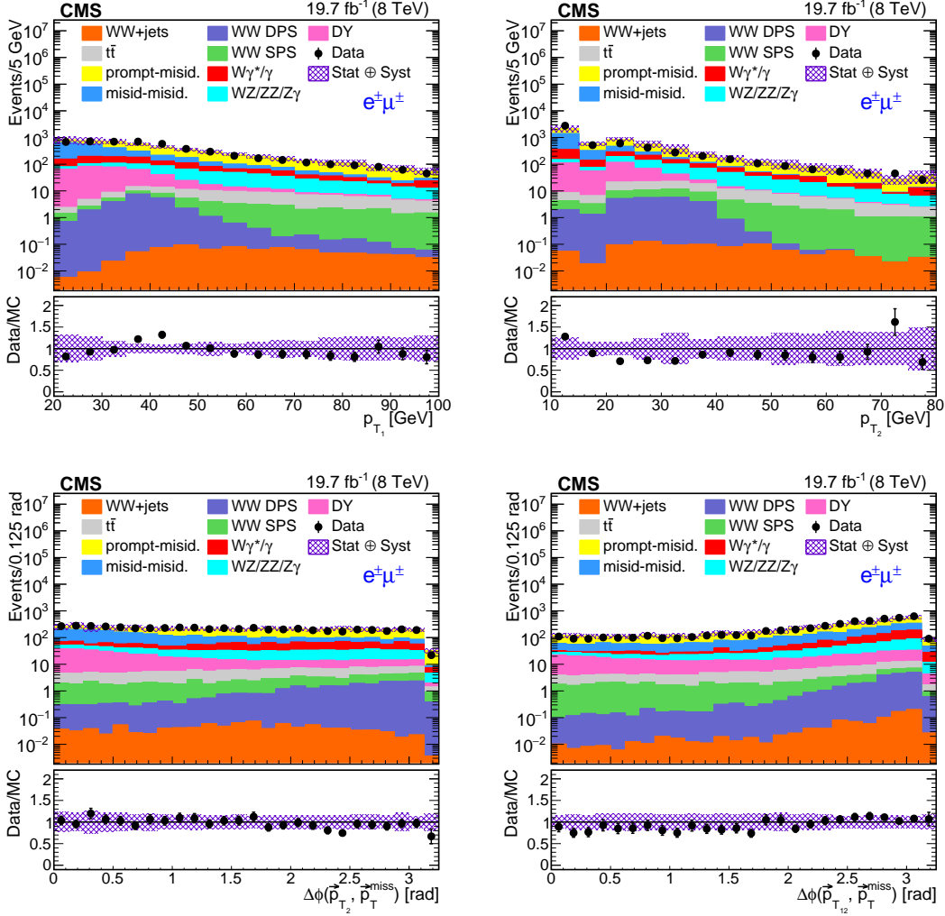
Figure 3: Distributions of the p_{T1} (top-left), p_{T2} (top-right), \Delta\phi(\vec{p}_{T2}, \vec{p}_T^{\text{miss}}) (bottom-left), and \Delta\phi(\vec{p}_{T12}, \vec{p}_T^{\text{miss}}) (bottom-right) variables for the electron-muon channel, after the same-sign WW selection criteria have been applied. Symbols and patterns are the same as in Fig. 2.
